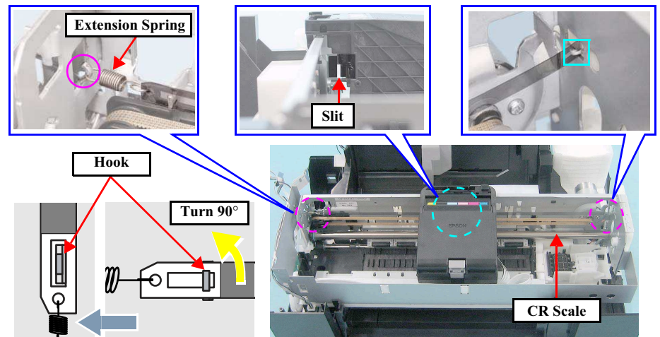
Figure 4-53. Removing the CR Scale
