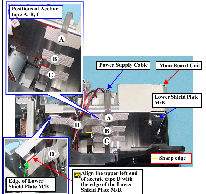
Figure 4-20. Routing the Cables
