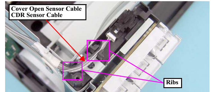
Figure 4-26. Installing the Panel Assy (1)
