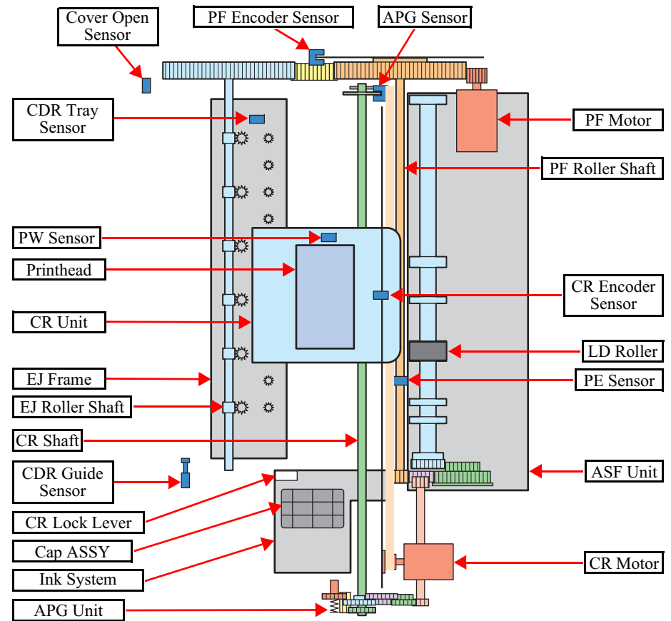
Figure 2-1. Printer Mechanism Diagram
