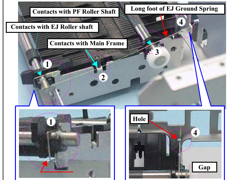
Figure 4-112. Attaching the EJ Ground Spring
