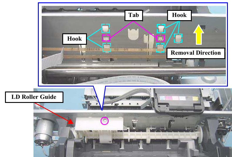
Figure 4-97. Removing the LD Roller Guide (1)
