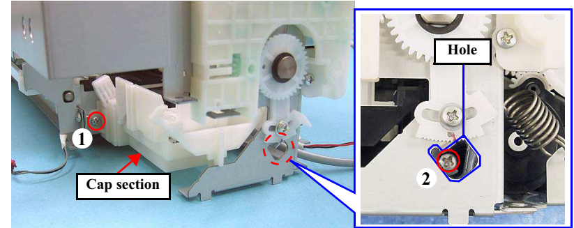
Figure 4-68. Removing the Ink System (1)
