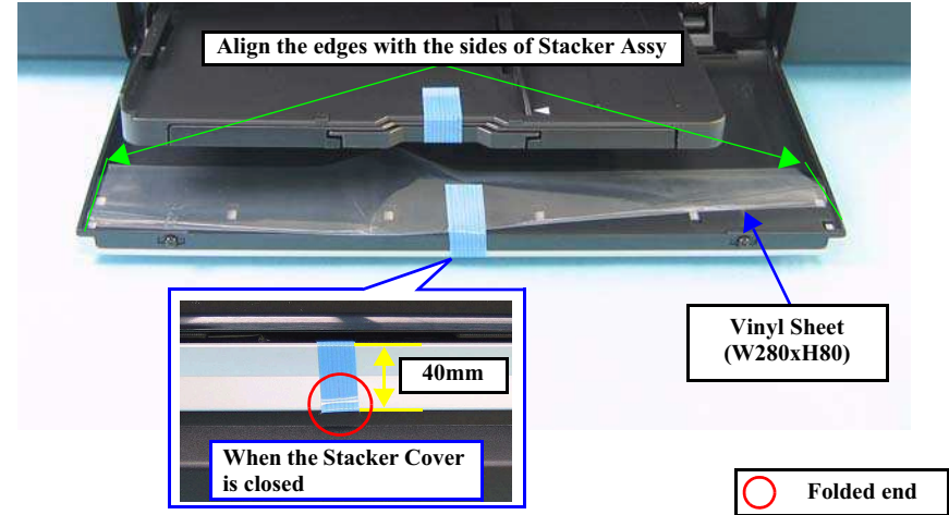
Figure 4-6. Securing the Stacker Cover
