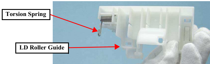
Figure 4-98. Removing the LD Roller Guide (2)
