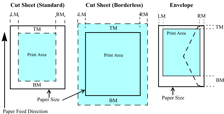
Figure 1-2. Printing Area
