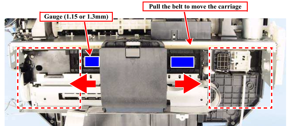
Figure 5-9. PG Adjustment 1
