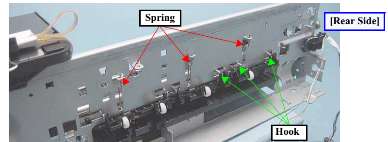
Figure 4-103. Removing the Upper Paper Guide (1)
