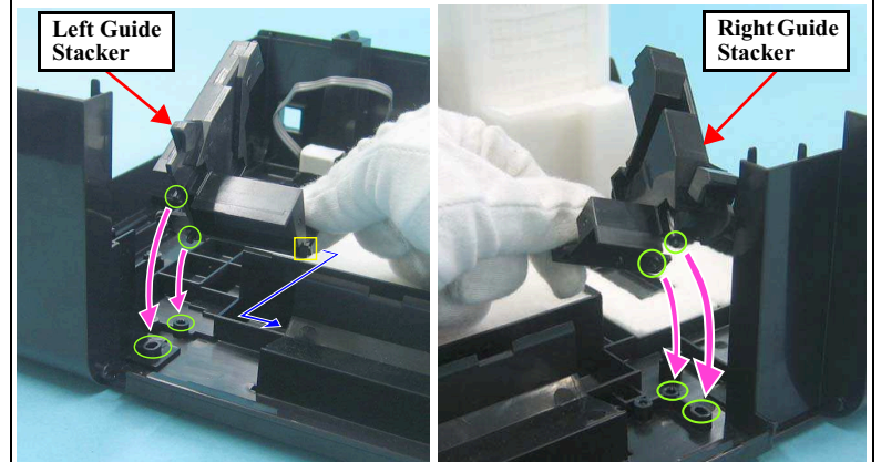
Figure 4-65. Installing the Left / Right Guide Stacker
