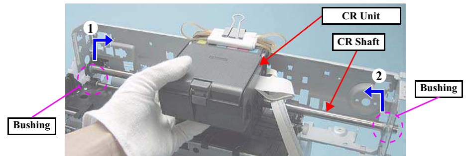
Figure 4-90. Removing the CR Unit (3)
