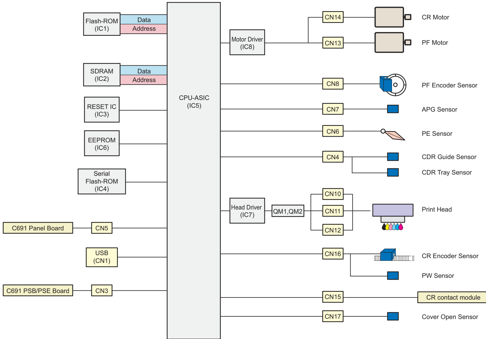
Figure 2-3. Circuit Block Diagram for R280/R285/R290
