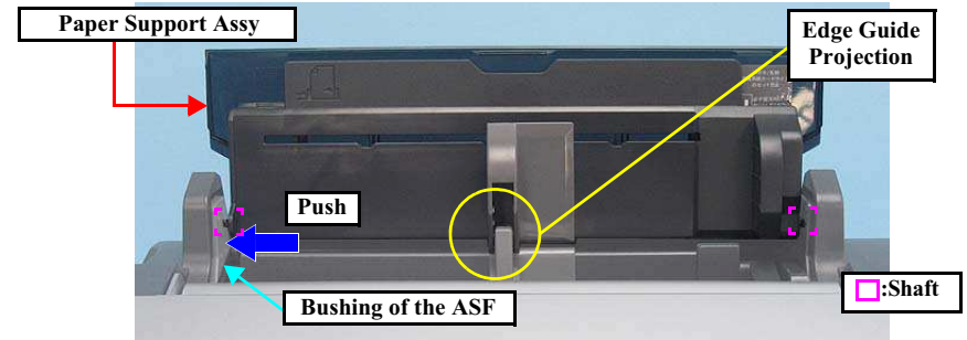
Figure 4-10. Removing the Paper Support Assy
