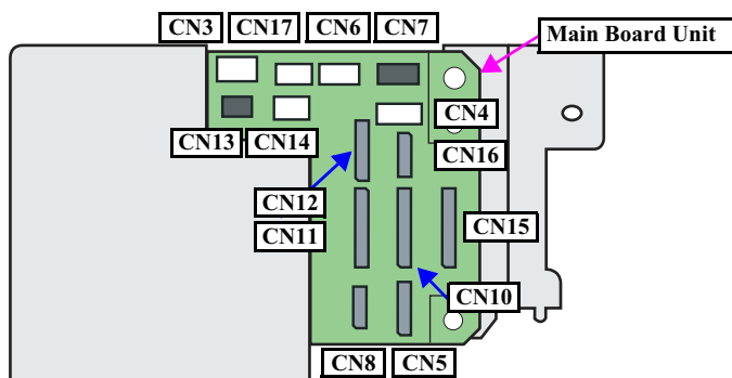
Figure 4-17. Connector layout of the Main Board
