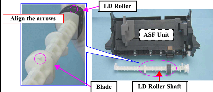
Figure 4-102. Reinstalling the LD Roller
