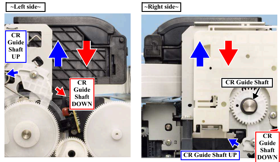
Figure 5-10. PG Adjustment 2
