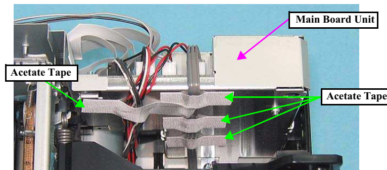
Figure 4-18. Removing the Main Board Unit (1)
