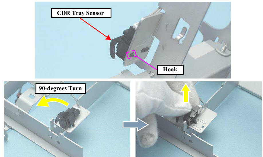
Figure 4-114. Removing the CDR Tray Sensor
