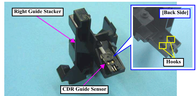
Figure 4-66. Removing the CDR Guide Sensor
