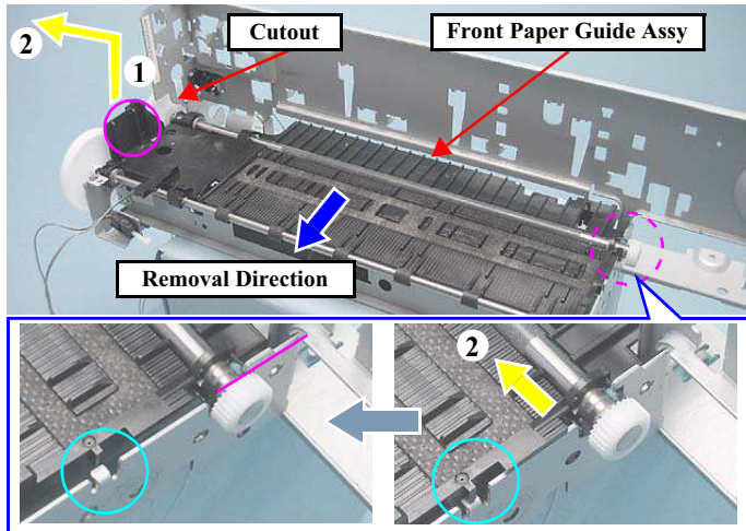
Figure 4-110. Removing the Front Paper Guide Assy
