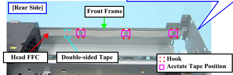
Figure 4-72. Removing the Head FFC
