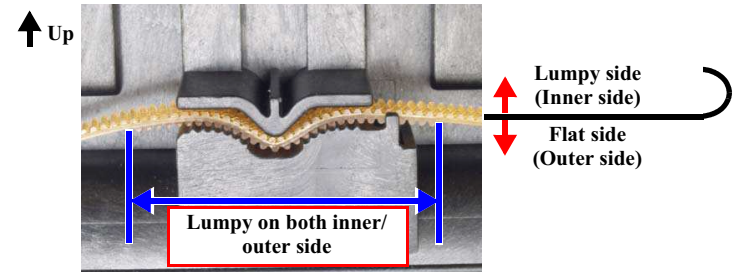
Figure 4-94. Reinstalling the Timing Belt
