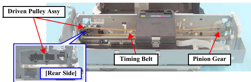
Figure 4-83. Removing the CR Motor (1)
