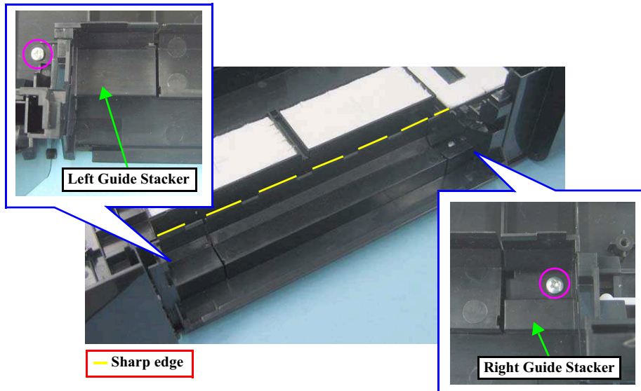
Figure 4-64. Removing the Left / Right Guide Stacker
