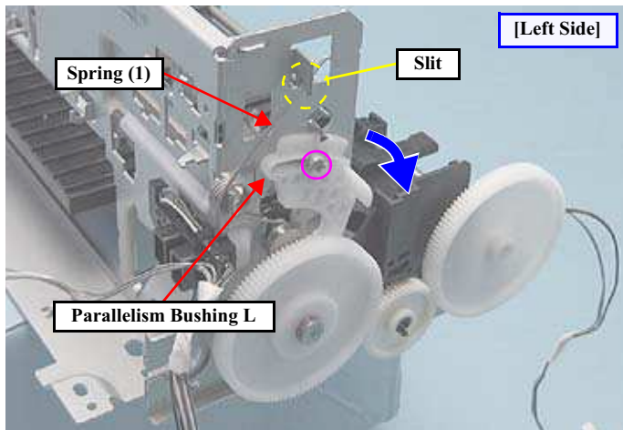
Figure 4-88. Removing the CR Unit (1)
