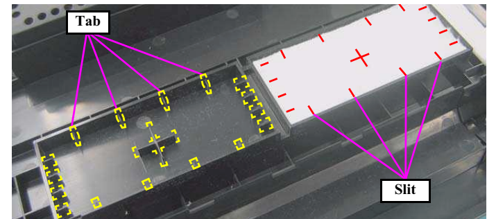
Figure 4-63. Installing the Waste Ink Pad
