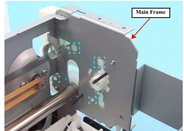
Figure 4-60. Reinstalling the APG Unit (4)
